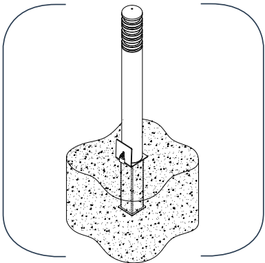
Removable Bollard Core BOL-RB-CORE 1350mm
