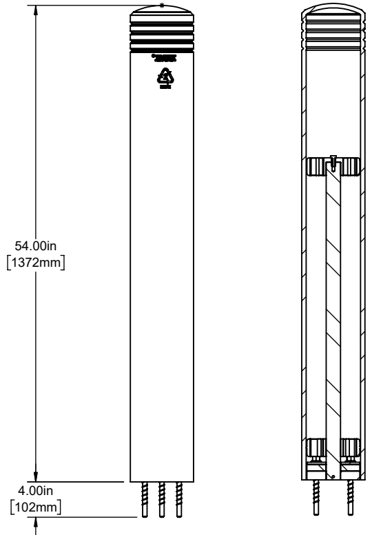
SECTION CB-CB
